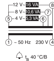
TS16/4-8-12
