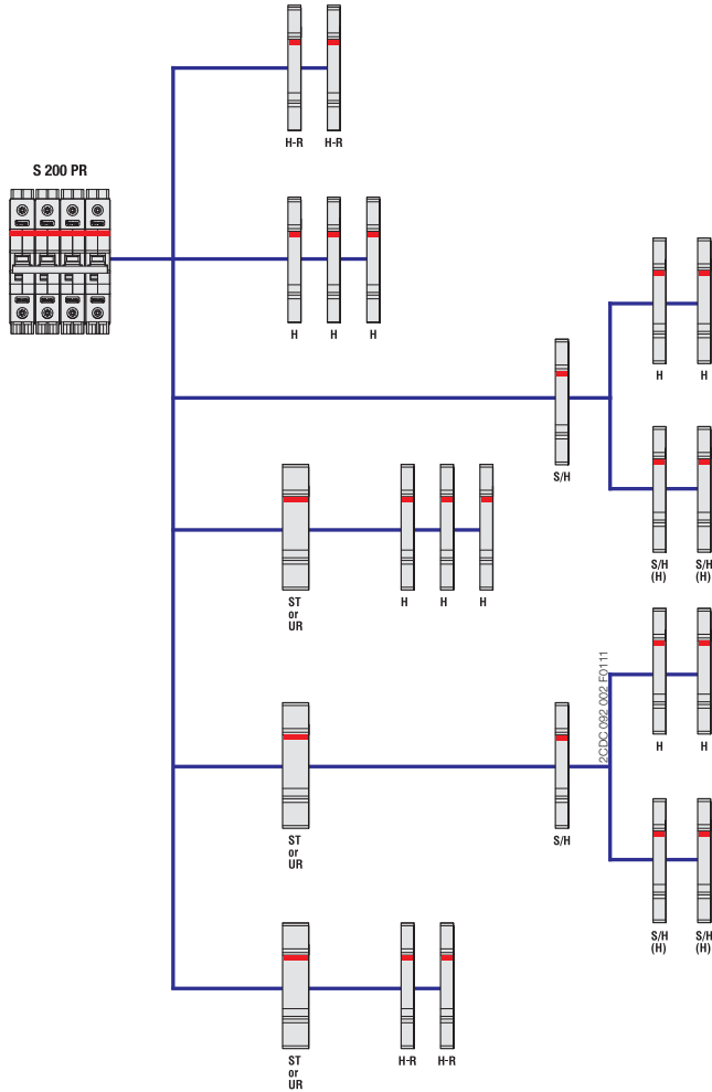
Combination of auxiliary elements with S 200 PR
