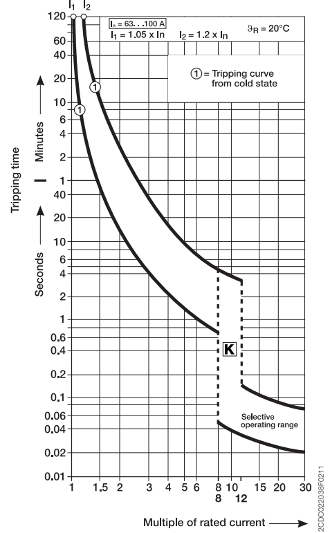
Characteristic K selective S 700 - 63 ... 100 A
