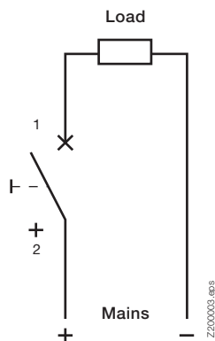
Connection diagram, single-pole (max. 125 V=) S401M-UCZ
