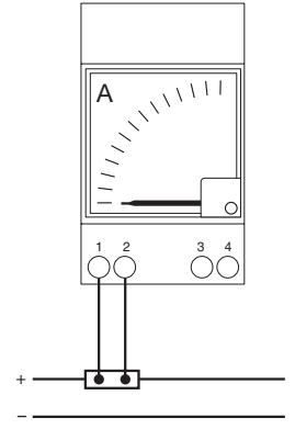
Indirect insertion using shunt
