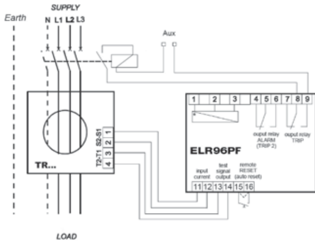
ELR96PF - shunt trip wiring
