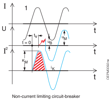
Oscillogram of short-circuit breaks on two circuit-breakers:
