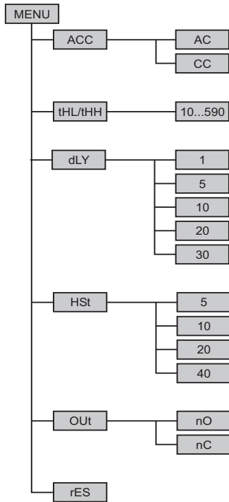
Voltmeters menu layout
