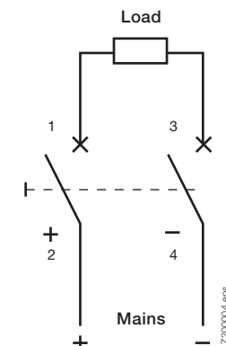
Connection diagram, two-pole (max. 250 V=) S402M-UCZ
