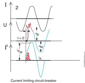
Short-circuit current
