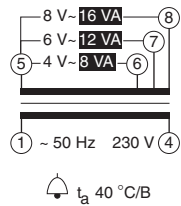
TS16/4-6-8
