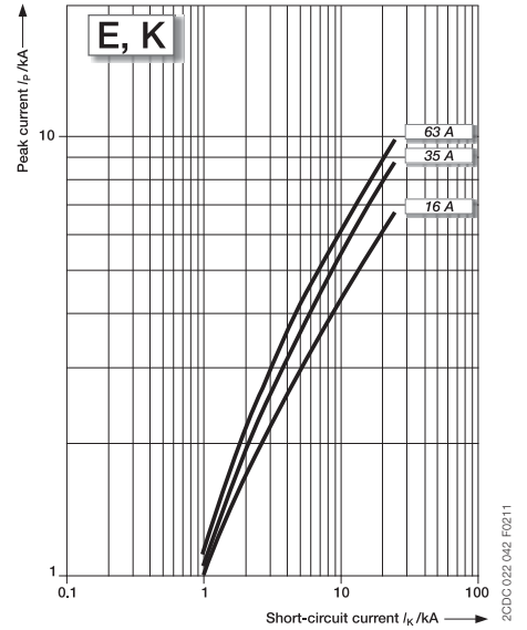
S 750 DR characteristic E_{selective}, K_{selective} let-through peak current ( I_{peak} )
