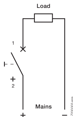
Connection diagram, single-pole (max. 125 V=) S401M-UCC
