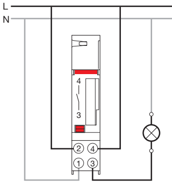
AT1, AT1-R
