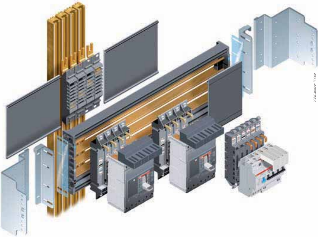
Unifix L
