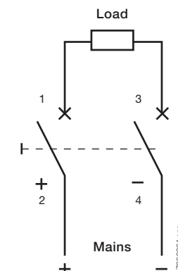
Connection diagram, two-pole (max. 250 V=) S402M-UCC
